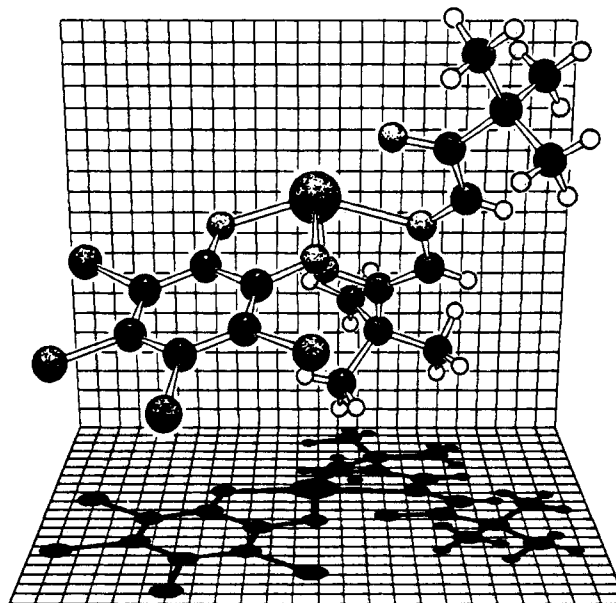
Figure 6. X-ray structure of DitBuADSbO· o -chloranil.
