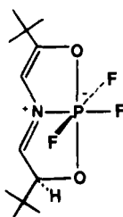
\text{DitBuADPO}\cdot\text{HF}_3
