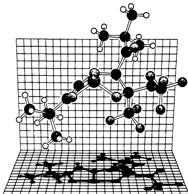
Figure 7. Structure of DitBuADPO·HFBA.
