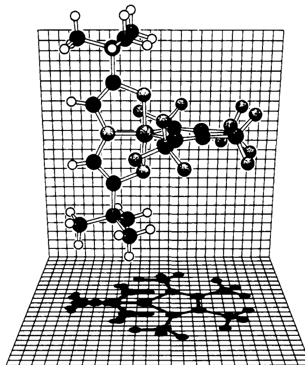
Figure 10. X-ray structure of DitBuADPO·2HFB.
