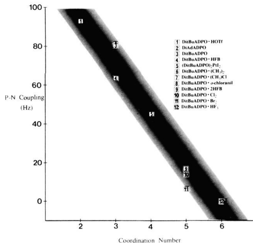
Figure 3. 31 P– 15 N couplings vs. coordination number.
