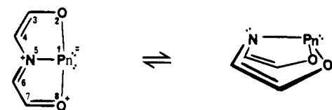
10-Pn-3
