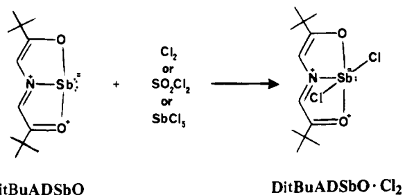
Figure 11. Structure of DitBuADSbO·Cl 2 .
